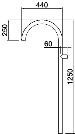
Colonna completa Complete shower column
